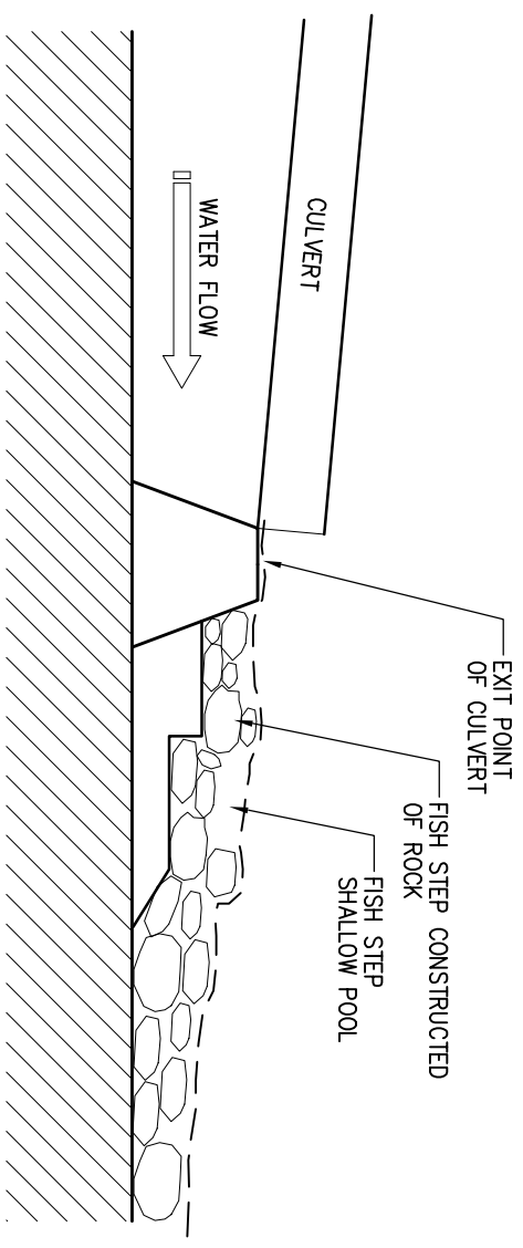
(c) CONCEPT FOR FISH SLOPE/STEP AT CULVERT OUTLET
